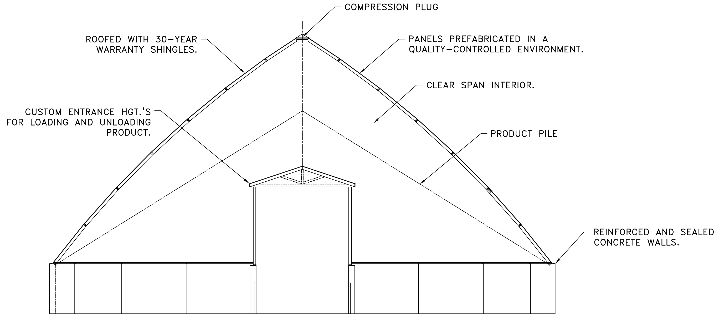
FRONT ELEVATION
